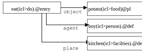
Fig. 2. Representation of a UNL expression.
